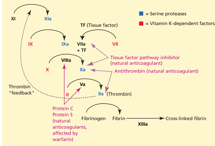
FIGURE 1. Contemporary coagulation cascade with inhibitors (natural anticoagulants).
