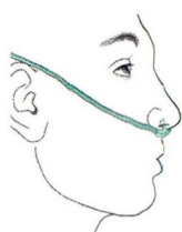
NASAL CANNULA
