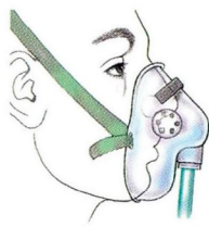
SIMPLE MASK
