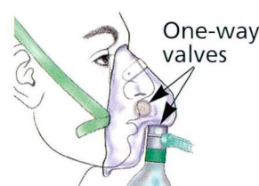
NONREBREATHING MASK
