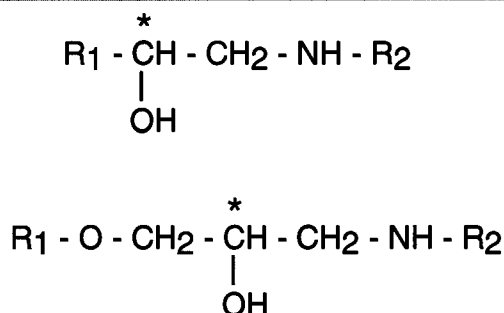
FIGURE 1. The aryethanolamines, (top) include labetalol, arotinolol, and amosulalol. The aryloxyisopropanolamines, (bottom) include celiprolol, nipradilol, bevantolol, and carvedilol. The asterisks show the position of the optic center of the compounds. Only labetalol is available in the United States.
