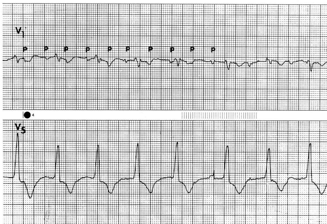
Fig. 3. Patient 3's ECG during follow-up stress test with his pacemaker programmed to below the intrinsic escape rate. Complete AV block is demonstrated with two simultaneously recorded leads, V1 and V5. The atrial rate (denoted as p ) is approximately 150 beats per minute. The ventricular response is approximately 80 beats per minute.
