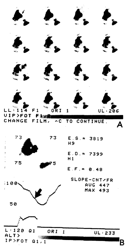
Fig. 4A. Postadriamycin gated left ventricular radionuclide study showing end-diastole (small black arrow) and end-systole (curved arrow). 4B. Postadriamycin computer printout showing a decrease in the ejection fraction to .48 and a decrease in the rate of ventricular emptying.
