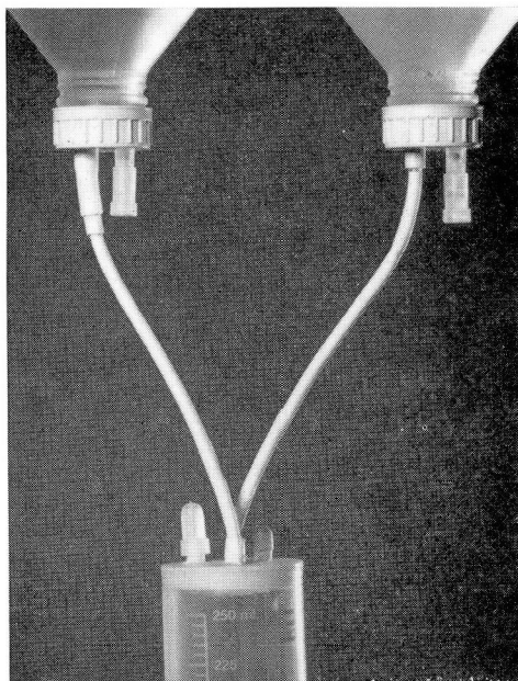
Fig. 2. Modified Soluset with second dispensing cap and sealed air vent in place.
