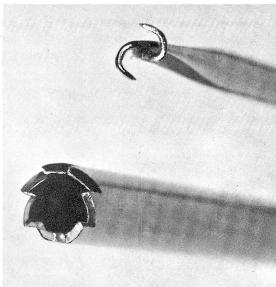
Fig. 1. Below, the serrated end of the Craig needle, and above, the S-shaped styler for removal of the plug of tissue.
