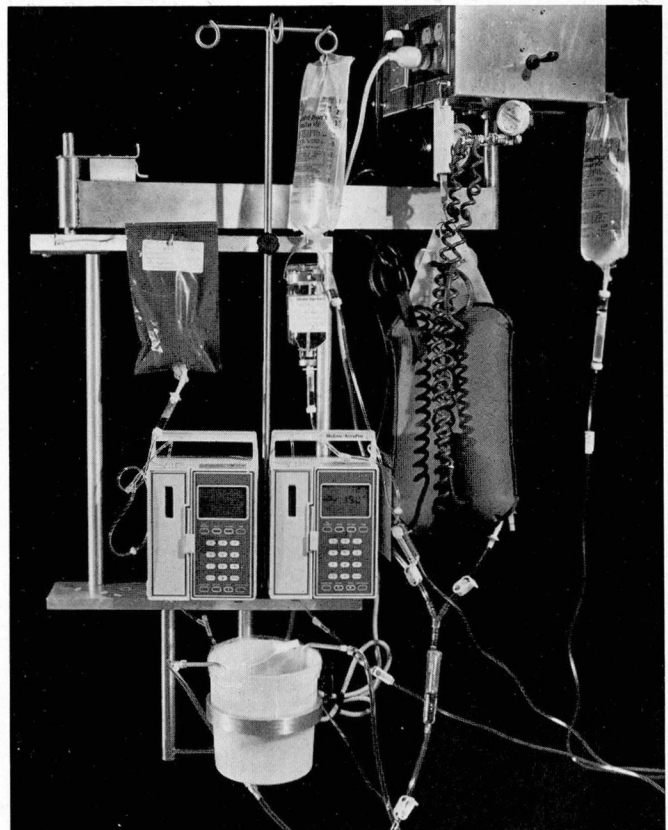
FIG. 3A. The infusion rack. 1 = the rack, 2 = ceiling-mounted column, 3 = rotating arm, 4 = rotatable detachable coupling, 6 = vertical bars for attachment of up to five infusion pumps, 7 = hooks for hanging infusion bags, 8 = valve handle used to control the internal pneumatic cylinder that determines column height, 9 = air-pressure regulator and manifold for operating pneumatic infusion pumps, 10 = electrical outlets, 11 = bracket and ice bucket used for the cardioplegia heat-exchange coil, 12 = additional stationary IV hooks, 13 = vertically adjustable IV post, and 14 = infusion pumps. FIG. 3B. The arm and rack as rotated for mounting onto the ICU bed. FIG. 3C. Infusion rack and column. The cardioplegia system is shown. Cold cardioplegia solution is pressurized by pneumatic infusion pumps supplied from the regulated air-pressure source, chilled by passage through an aluminum coil in the ice bucket, and passed through a bubble trap.
