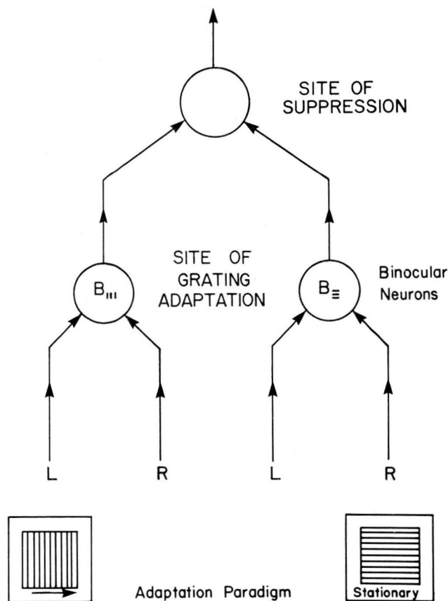
Fig. 2. Schematic diagram of the adaptation paradigm to study the effect of retinal rivalry on the MAE. A moving vertical grating is presented to the left eye while a rivalrous stationary horizontal grating is presented to the right eye. The two stimuli affect different binocular neurons.
